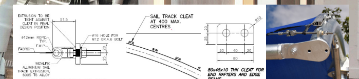
Proprietary Fixing Details and Connections
